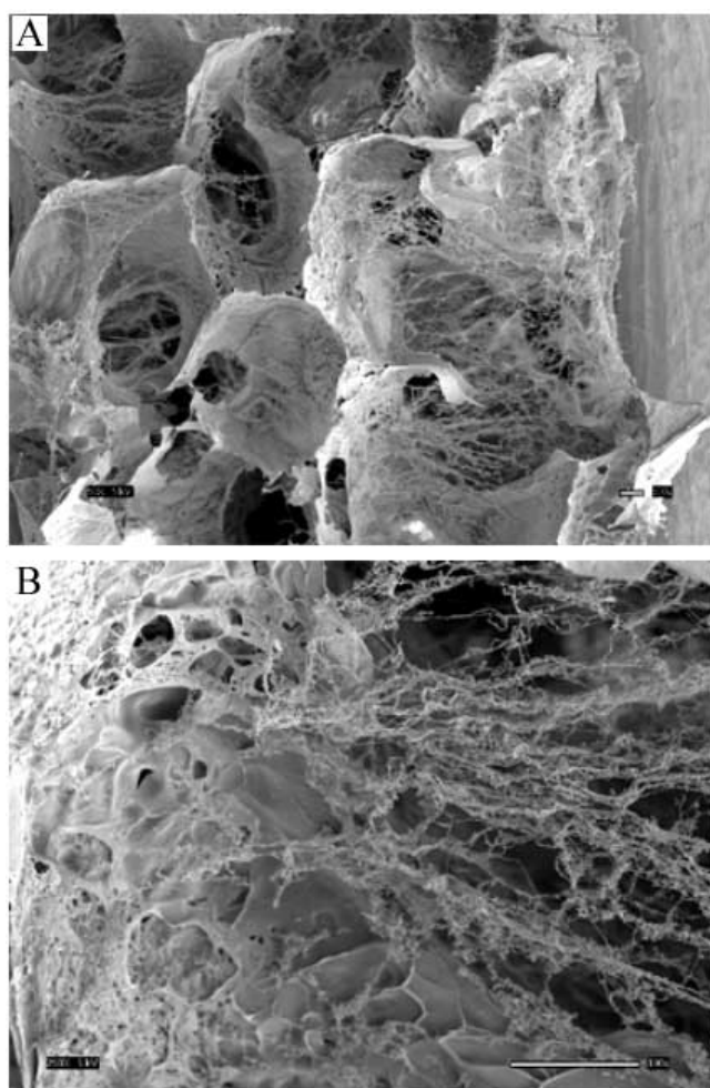
Figure 8. Cryo SEM images of a hydrated PAN/P(AM-co-SPAK) SPIH (A) and an area near the pore walls of the SPIH (B). The magnifications of the micrographs A and B are \times 50 and \times 250 , respectively. The scale bars are both 100\ \mu\text{m} .
