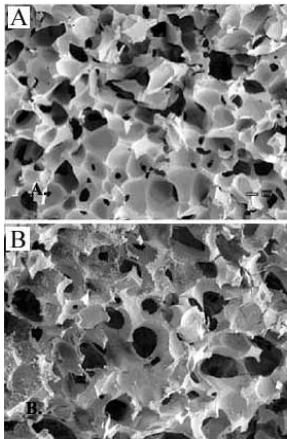
Figure 7. Scanning electron micrographs of P(AM-co-SPAK) SPH (A) and PAN/P(AM-co-SPAK) superporous IPN gel (B) in the dry state. The magnification of the micrographs is ×50, and the scale bar indicates 100 μm.
