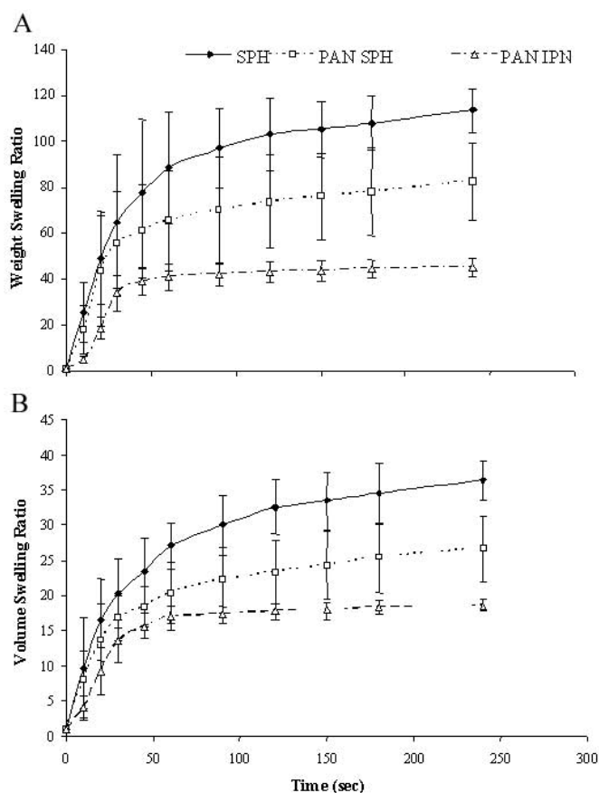
Figure 4. Weight swelling curves (A) and volume swelling curves (B) of 3 types of P(AM-co-SPAK) hydrogels (n=3, mean ± SE).
