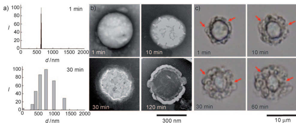
Figure 2. a) Size distribution of GGPNPs incubated in PBS at 37°C for 30 min measured using DLS. b) TEM micrographs of GGPNPs hydrolyzed in PBS for 2 h at 37°C. c) Optical micrograms of gas-generating profiles of microsized GGPNPs (6–8 μm) incubated in PBS at 37°C for 1 h (arrows indicate gas-generating bubbles). Original magnification is ×400.
