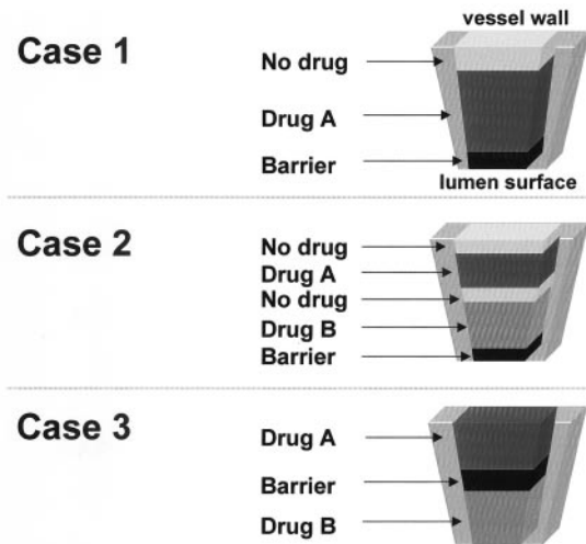
Figure 6. Schematic of 3 polymer/drug layering combinations in a strut hole.
