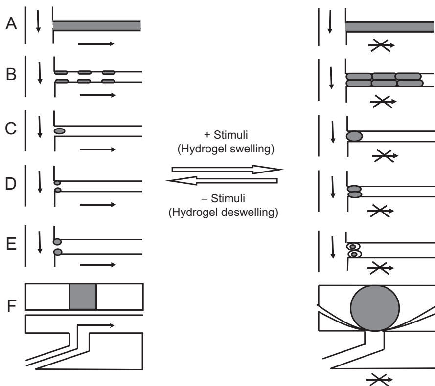
Fig. 12. Schematic for hydrogel swelling-modulated flow control via smart channels and valves: (A) and (B) represent smart channel designs—with a hydrogel strip (A), with a patterned array of hydrogel posts (B); (C)–(E) represent smart valve designs—with a single post (C), multiple posts (D), and multiple jacketed posts (E); (F) represents a hybrid hydrogel-flexible diaphragm (e.g., PDMS) valve where the expansion of the hydrogel deforms the diaphragm, reminiscent of the deformation of a bimetallic strip on heating (modified from [281]).
