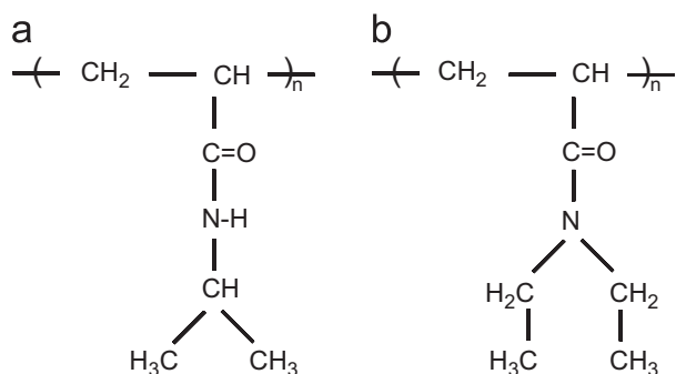
Fig. 7. Chemical structures of thermally responsive poly( N -substituted acrylamide)s. (a) poly( N -isopropylacrylamide); (b) poly( N,N' -diethylacrylamide). These polymers exhibit LCST phase transition. Notably, a common characteristic of most LCST polymers is the presence of hydrophobic alkyl groups.
