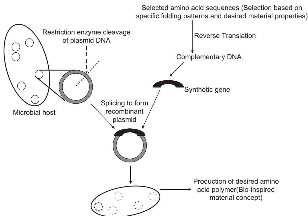
Fig. 4. Overview of the protein engineering methodology (modified from Ref. [321]).
