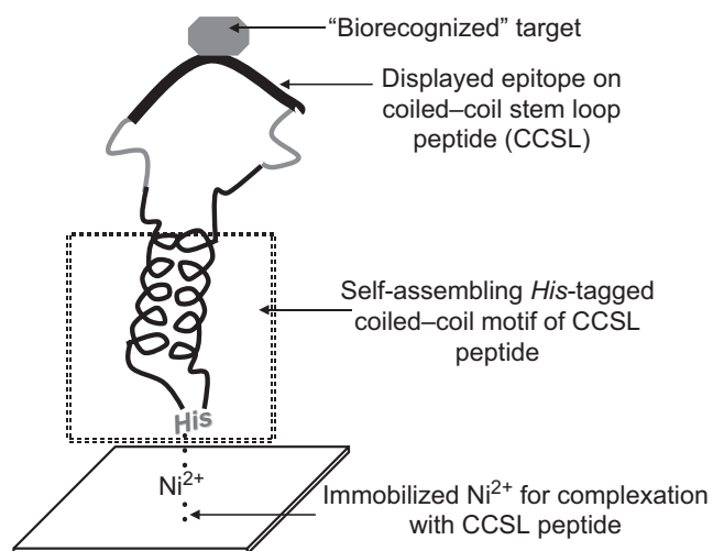
Fig. 6. Biorecognition of target via the displayed epitope on a coiled-coil stem-loop (CCSL) peptide (modified from Ref. [82]).
