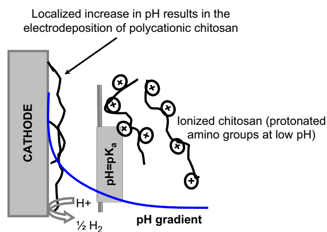
Fig. 13. Directed assembly of chitosan in response to locally applied electrical stimuli, i.e., electrodeposition of chitosan; the thickness and other properties of the electrodeposit can be controlled by varying electrochemical parameters (modified from [287]).
