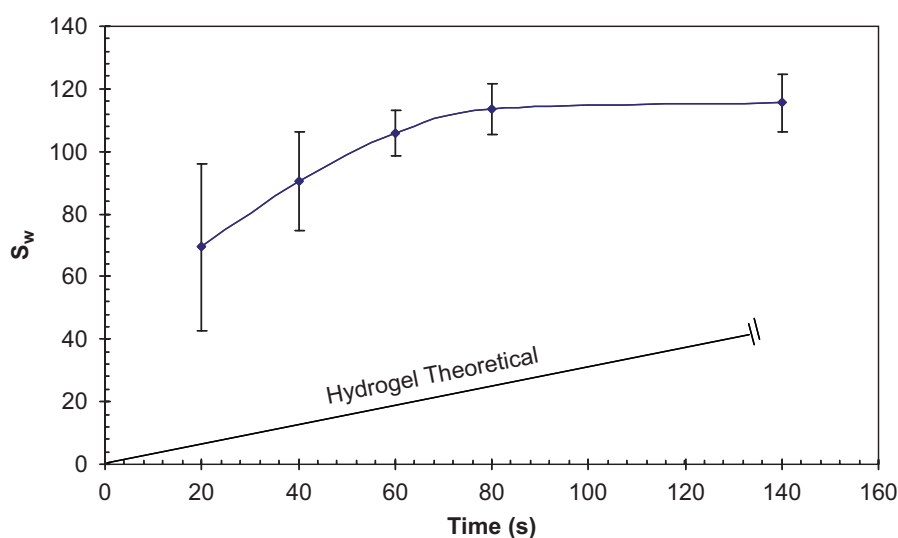
Fig. 3. An example of swelling ratio ( S_w ) as a function of time for SPHs made of acrylic acid (AA) and acrylamide (AM). The straight line representing “hydrogel theoretical” describes a typical example of the increase in S_w with time for a hypothetical non-porous hydrogel.
