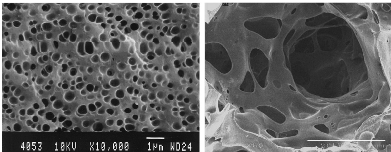
Fig. 2. Scanning electron micrographs of SPHs with pore sizes less than 1 \mu\text{m} (left) and larger than 1 mm (right). The scale bars are 1 \mu\text{m} and 1 mm for the pictures on the left and right, respectively.
