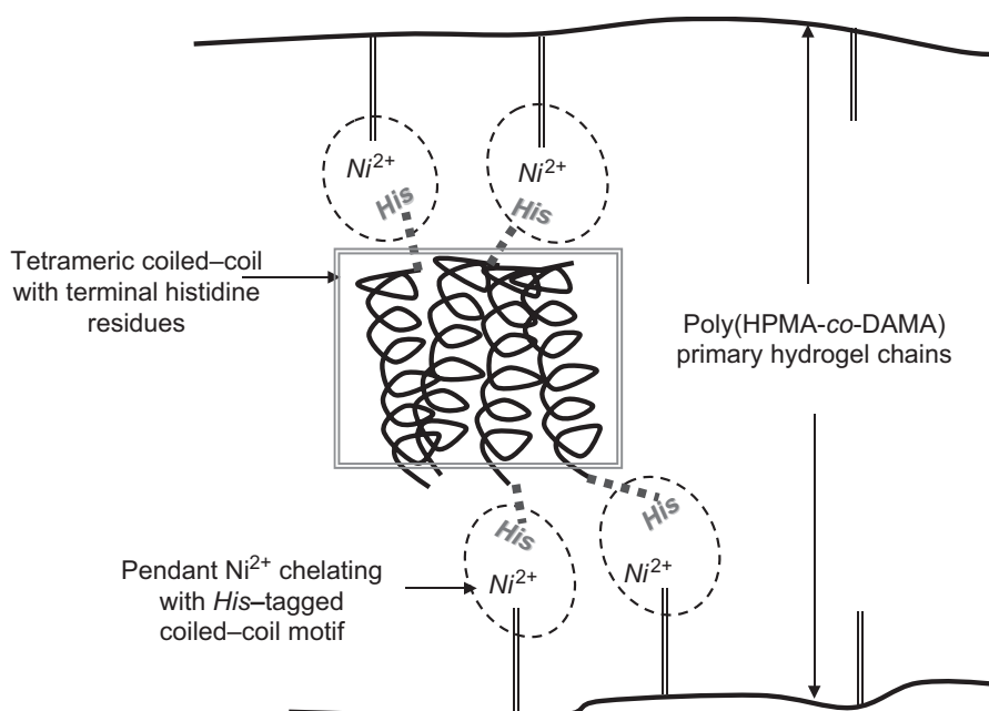
Fig. 5. Schematic of a hybrid hydrogel assembled from histidine-tagged coiled-coil proteins and the synthetic polymer, poly(HPMA-co-DAMA). The pendant iminodiacetate groups from DAMA complex with \text{Ni}^{2+} , to which the terminal histidines of the coiled-coil tetramer (not drawn to scale) are attached. The tetrameric, self-assembling coiled-coil motif, crosslinking the primary hydrogel chains, consist of two parallel dimers associating in an antiparallel fashion, and constitute only one of the several possible conformations of coiled-coil proteins (modified from Ref. [92]).
