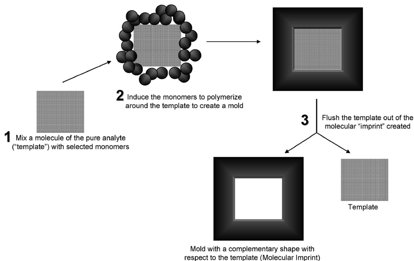
Fig. 11. Schematic for the fabrication of molecularly imprinted polymers (MIPs) (modified from Ref. [249]).
