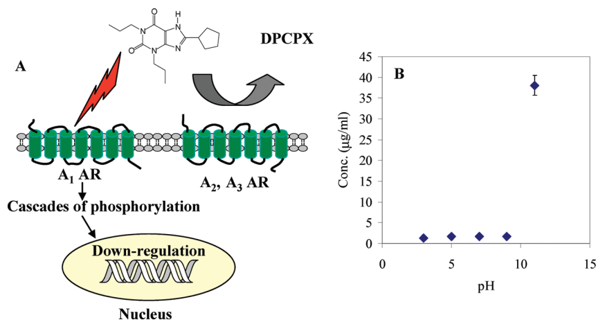
Figure 1. Chemical structure and pharmacological action of 1,3-dipropyl-8-cyclopentyl xanthine (DPCPX) (A), and the pH-dependence solubility of DPCPX in water (B).
