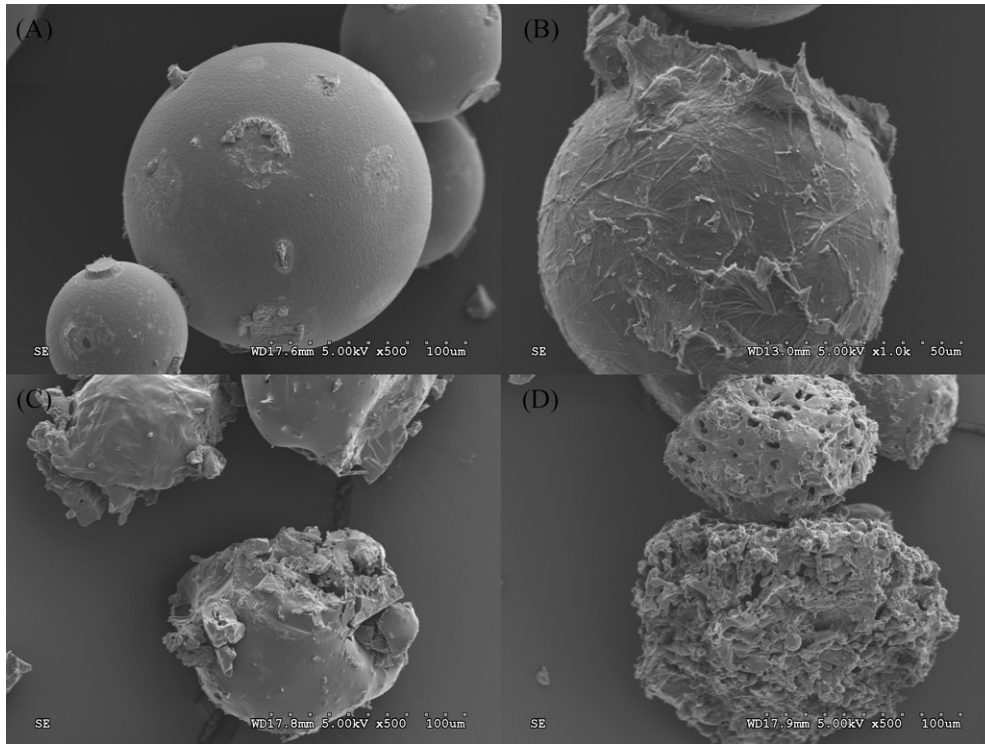
Fig. 7. Scanning electron micrographs of 5% paclitaxel-loaded PLGA microspheres blended with, A: No diblock copolymer, B: 22% MePEG-b-PDLLA, C: 27% MePEG 17 -b-PCL 5 and D: 32% MePEG 17 -b-PCL 10 following 10 weeks incubation in PBS at 37 °C.
