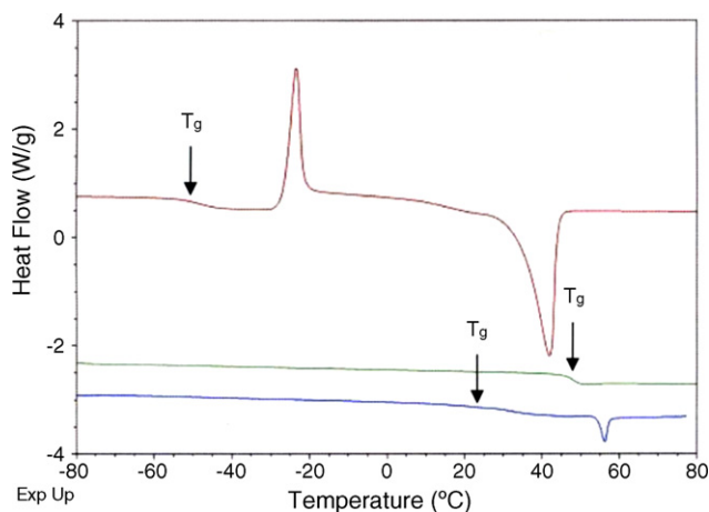
Fig. 4. Thermal analysis: representative DSC heating curves ( 10^\circ\text{C}/\text{min} ) for MePEG-b-PDLLA diblock copolymer loaded PLGA microspheres. Top curve: PDLLA diblock copolymer alone, middle curve: PLGA alone and bottom curve: MePEG-b-PDLLA diblock copolymer (22%) loaded PLGA microspheres.
