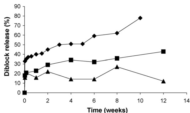
Fig. 6. Release of diblock copolymers from PLGA microspheres loaded with 22% (w/w) MePEG-b-PDLLA ( \blacklozenge ), 27% (w/w) MePEG 17 -b-PCL 5 ( \blacksquare ) and 32% (w/w) MePEG 17 -b-PCL 10 ( \blacktriangle ) as determined by quantitative GPC.
