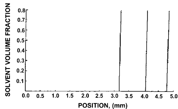
Fig. 30. Solvent volume fraction, f_s as a function of position, x . The polymer molecular weight was M = 40\,000 and t_{rep} = 1000 s. The position x = 0 is the center of the slab. The time increment starting from the first curve on the right is D_t = 1000 s. (Adapted from Ref. [105].)
