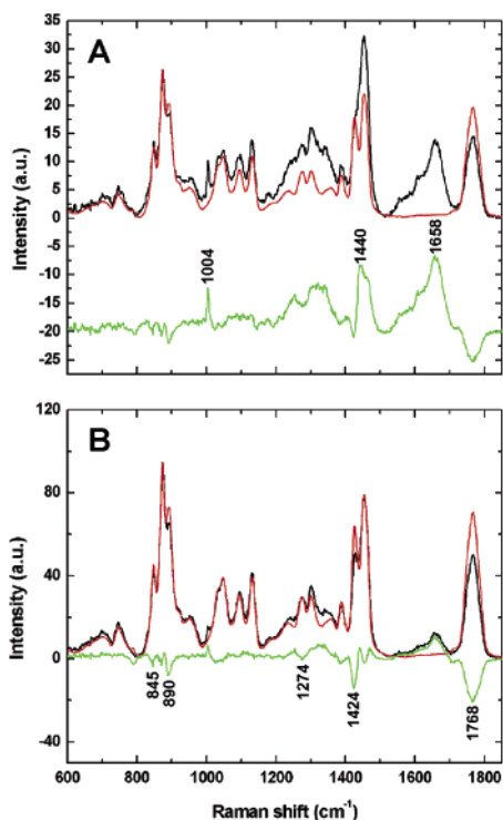
Figure 2. Raman spectra (in black) of the low- (A) and high-intensity (B) regions of the PLGA microsphere in Figure 3D. Pure PLGA is shown in red, and difference spectra (after scaling to the 875 \text{cm}^{-1} band) in green. Note the negative band at 1768 \text{cm}^{-1} (indicating a decrease in the number of ester bonds) and the negative bands specific for glycolic acid at 845, 890, 1274, and 1424 \text{cm}^{-1} . 11
