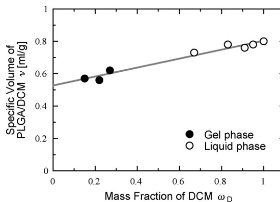
Fig. 3. Relationship between specific volume of PLGA/DCM solution and mass fraction of DCM.
